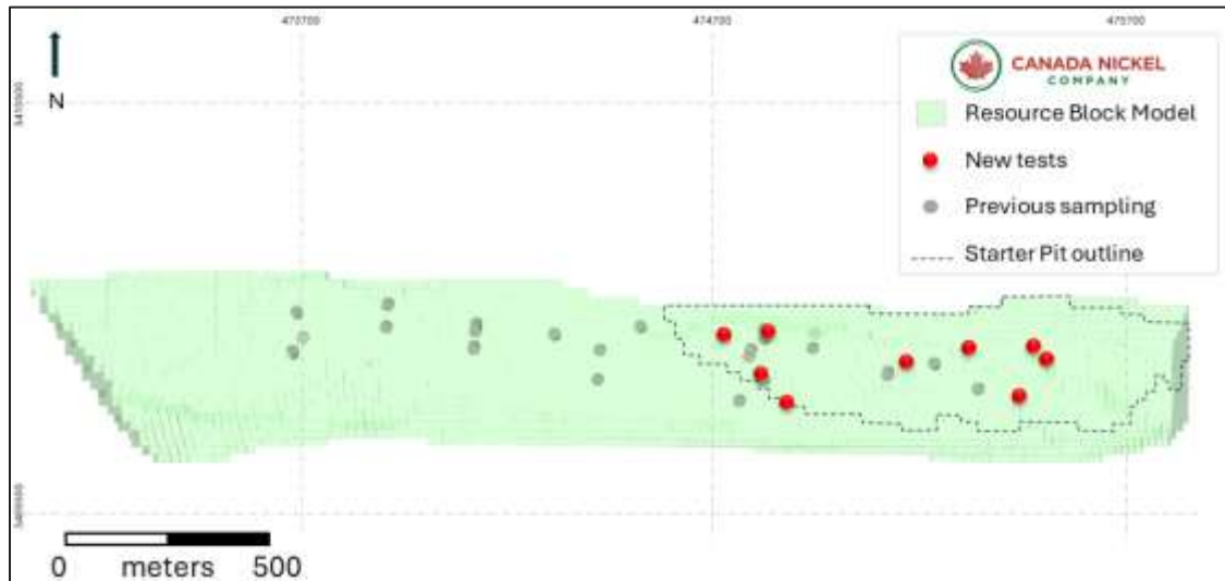
Figure 1. Crawford Nickel Sulphide Project - East Zone Open Cycle Tests
